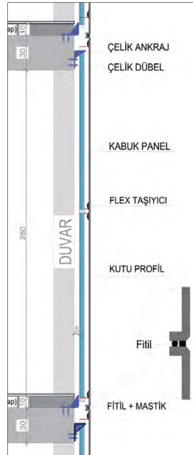
Panel Kesiti Panel Section
