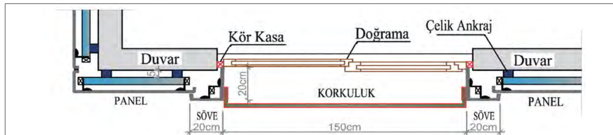
Panel Kesiti Panel Section
